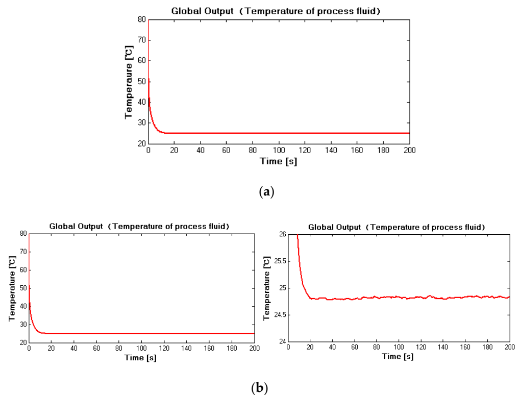
Figure 4. (a) Measured T_H (noise-free situation) in case 1; (b) measured T_H (noise-corrupted situation) in case 1.
