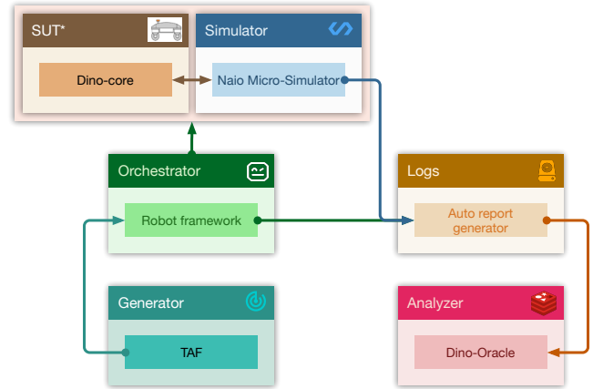
Figure 4: Testing architecture for Dino.
