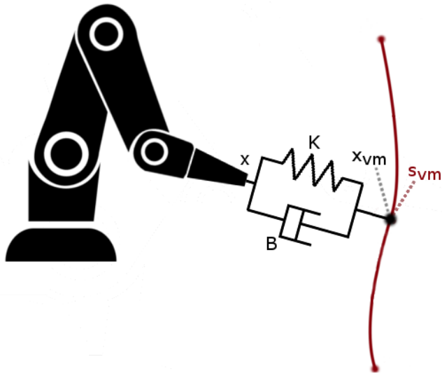
Fig. 2: Virtual mechanism representation. The red curve represents the possible configurations of the virtual mechanism in the Cartesian space X_{vm} , and because of the spring-damper system linking, it represents the allowed configurations of the robot end-effector X . The current position of the virtual mechanism is described by its parameterized space by the parameter s_{vm} \in \mathbb{R} .
