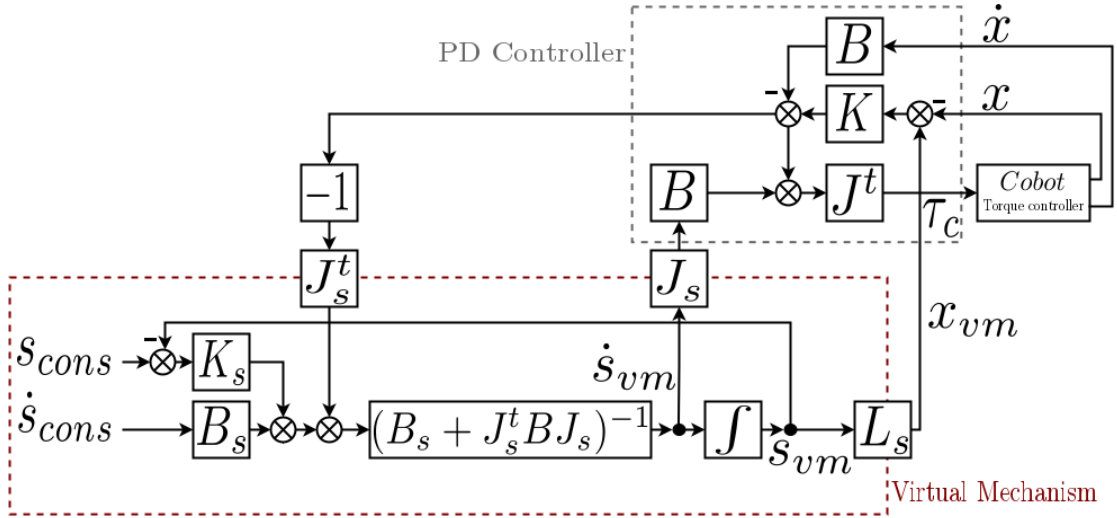
Fig. 4: Control law scheme of a 1-DOF virtual mechanism.
