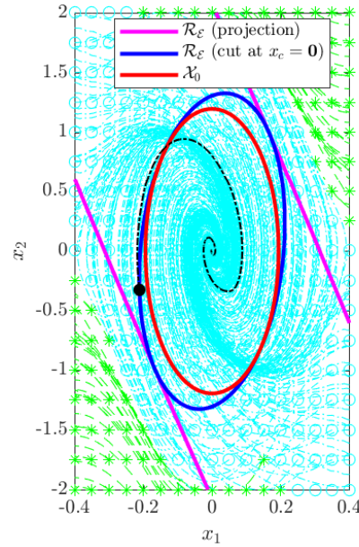
Figure 5: \mathcal{R}_{\mathcal{E}} and \mathcal{X}_0 = \mathcal{E}(R, 1) with R_{11} = \text{diag}\{26.60, 0.70\} .
