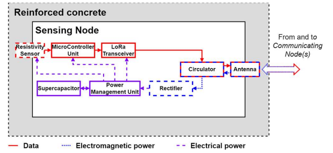
Fig. 2. Block diagram of the architecture of the Sensing Node dedicated to the measurement of the electrical resistivity of concrete.
