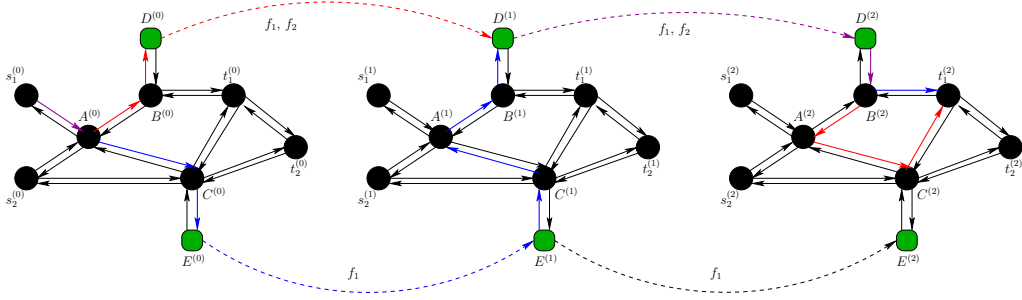
Figure 2: Expanded network for the example of Figure 1. The artificial edges between consecutive layers are shown with dotted lines. Two feasible paths for the demand from node s_1 to node t_1 are shown, with blue-coloured edges for the first one and with red-coloured edges for the other one (common edges are purple-coloured).
