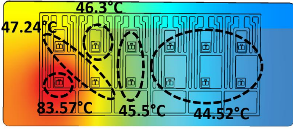
Figure 5. Illustrations of clusters for M1 ON P=50W and ambient temperature T_{amb}=40^{\circ}\text{C}
