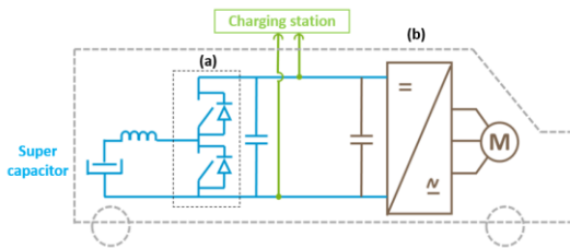
Figure 1. Illustration of the application (a) DC-DC converter (b) power train inverter
