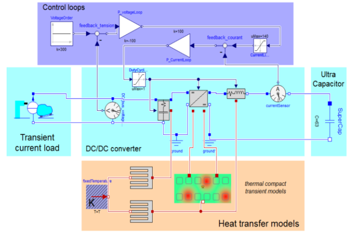
Figure 9. Modelica modelling of the electrical bus
