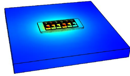
Figure 3. Simulation of the power module with optimized equivalent heatsink
