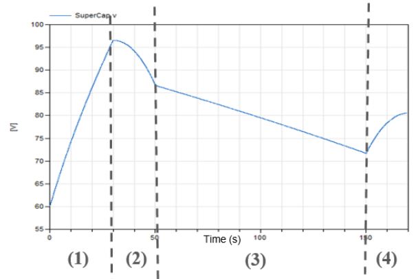
Figure 10. Supercapacitor voltage variation during the mission profile (1) supercapacitor charge (0-30s) (2) bus acceleration (30s-50s) (3) constant speed phase (50s-150s) (4) braking phase (150s-170s)
