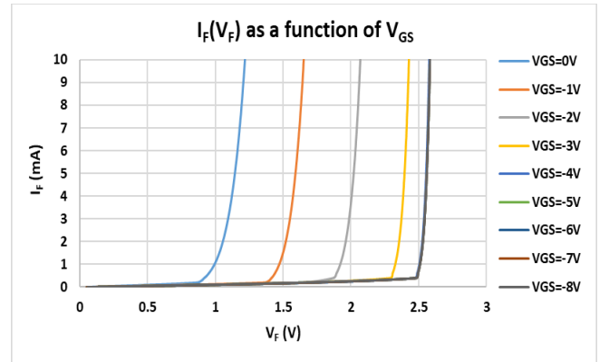
Fig. 6. I_F(V_F) as a function of the gate bias voltage V_{GS}
