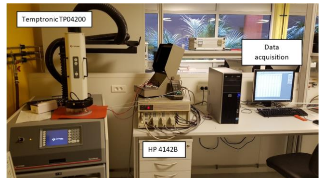
Fig. 3. Electrical test bench for power module characterization.
