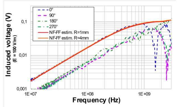
Fig. 13. Comparison between measurements of the induced voltage on a microstrip line terminated by 50-Ω loads for 4 orientations in GTEM cells, and estimation based on NFSI done at two different scanning heights
