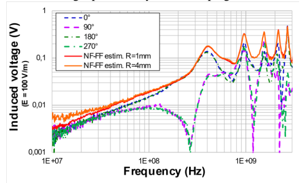
Fig. 14. Comparison between measurements of the induced voltage on a microstrip line terminated by 150-Ω and 10 pF loads for 4 orientations in GTEM cells, and estimation based on NFSI done at two different scanning heights
