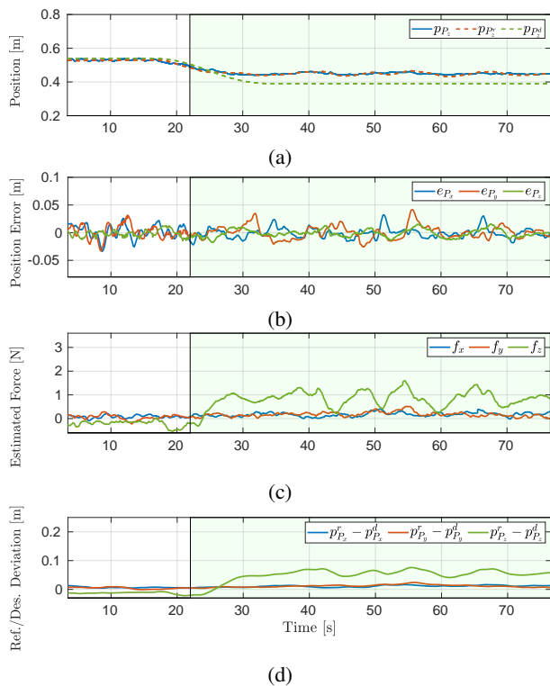
Fig. 5: Unexpected-collision interaction: 5(a) vertical actual platform position \mathbf{p}_P in solid lines, desired position \mathbf{p}_P^d and admittance reference \mathbf{p}_P^r in dashed lines. 5(b): position error e_P . 5(c): forces applied to the platform before and throughout the collision. 5(d): difference between the pre-planned trajectory and the references produced by the admittance filter.
