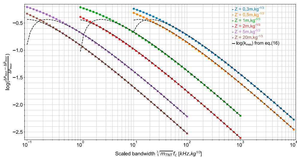
Figure 6. Estimation accuracy (\Delta P_{MAX} - \Delta \hat{P}_{MAX}) / \Delta P_{MAX} on the overpressure peak as a function of the scaled bandwidth \sqrt[3]{m_{TNT}}f_c for various scaled distances. Results are obtained for the side-on overpressure measurement and surface bursts.
