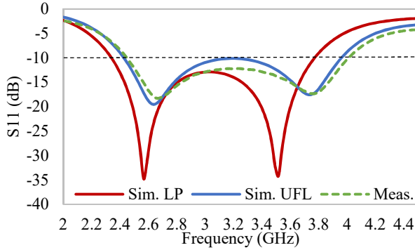
Fig. 10. Comparison of the simulated and measured return loss of the printing antenna.
