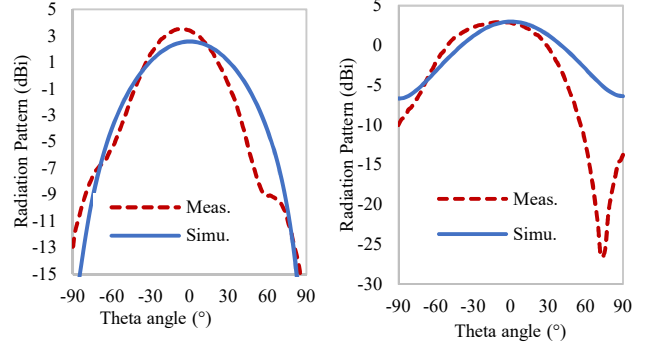
Fig. 12. Comparison of the measured and simulated radiation pattern in the E-plane ( \Phi = -90^\circ ) at 2.45 GHz (left) and 3.41 GHz (right).
