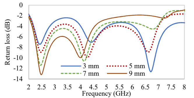
Fig. 3. Simulated return loss of antenna A2 with different Y_2 values.
