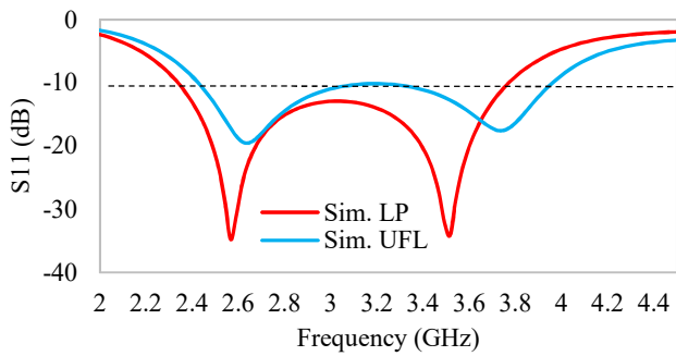
Fig. 6. Simulated antenna return loss with and without U.FL connector.
