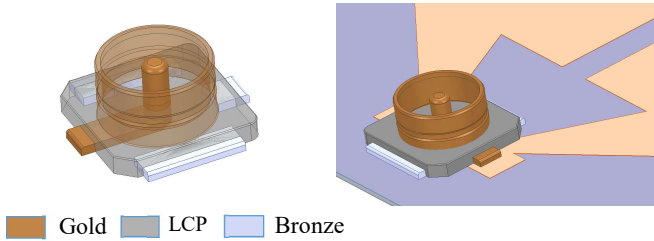
Fig. 5. (a) 3D model of the U.FL connector and materials assignment ; (b) Connector placement on the antenna feed pad.
