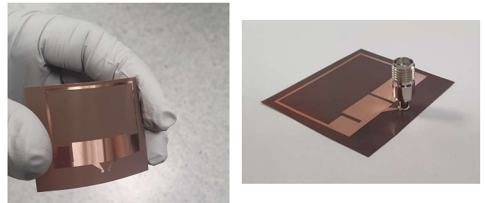
Fig. 8. Photo of the manufactured antenna in cleanroom and with U.FL connector and SMA adaptor mounted.
