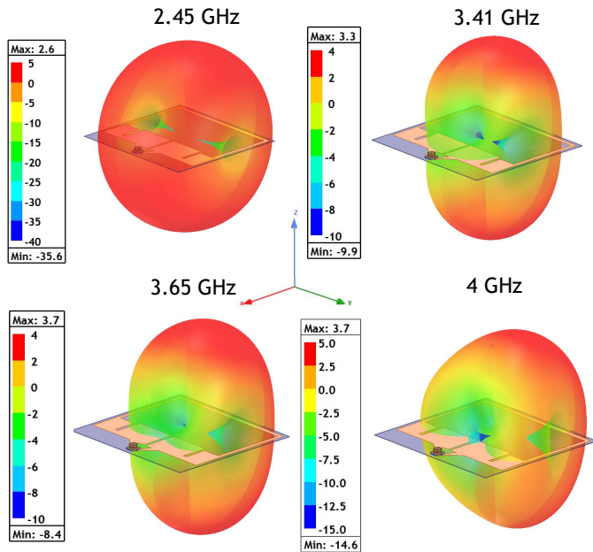
Fig. 7. Simulation of the 3D radiation pattern of the proposed antenna at different frequency.
