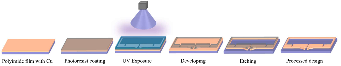
Fig. 9. Schematic representation of the photolithographic process.
