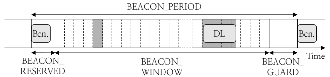
(b) LoRaWAN Class B
