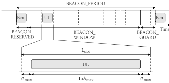
Fig. 4: LoRaSync beacon period and slot structure.
