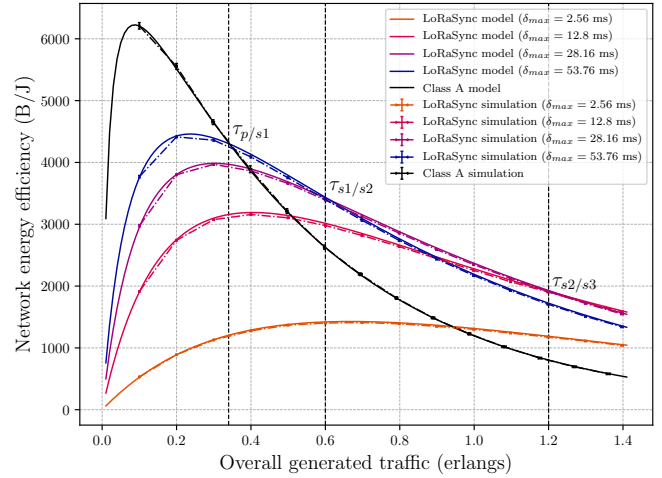
Fig. 6: Energy efficiency model and simulation results
