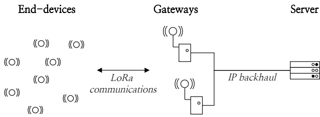
Fig. 1: LoRaWAN topology
