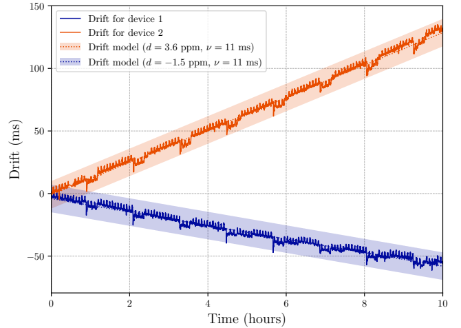
Fig. 3: Device drift measurements
