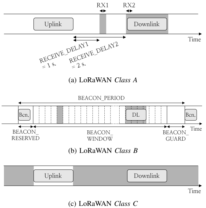
Fig. 2: LoRaWAN classes medium access
