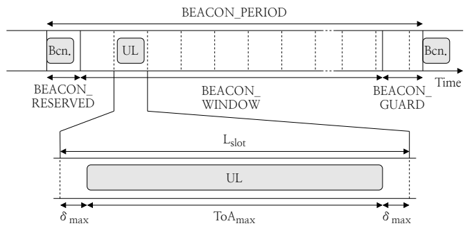
Fig. 4: LoRaSync beacon period and slot structure.
