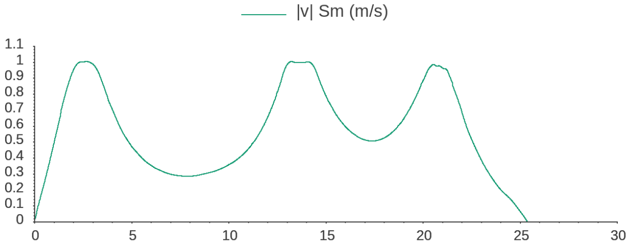
Figure 4: Magnitude of the drone's speed using BSpline composed of many iterations of KHAOS in the scenario with two humans.
