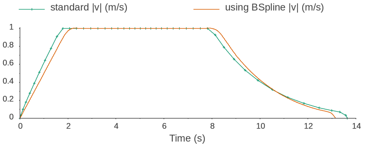
Figure 2: Magnitude of the drone’s speed before (green) and after (orange) using BSpline in the KHAOS output in the scenario where the drone approaches a human from the front in a straight line.
