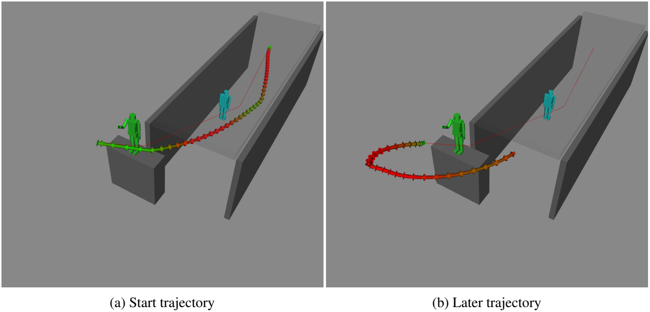
Figure 3: Trajectory execution in a two-humans scenario. a) First trajectory generated by KHAOS, the drone starts by navigating in the corridor. b) A few iterations later, after passing the blue human in the corridor. Red line: represents initial path before smoothing using BSpline. Red arrows: highest speed magnitude. Green arrows: lowest speed magnitude.
