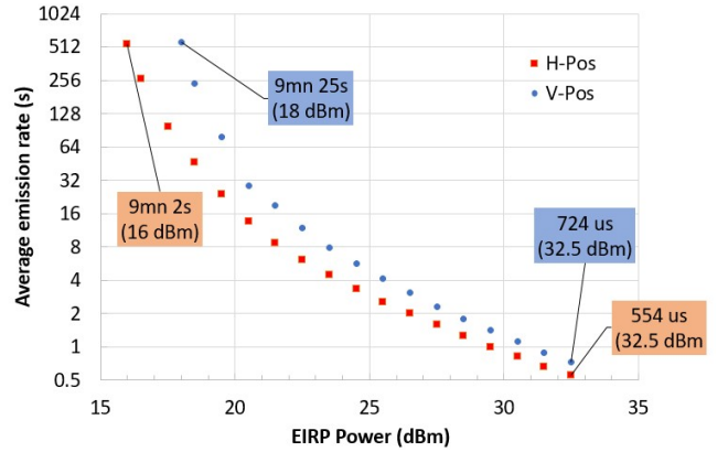
Fig. 6. Average emission rate of the tag in localisation mode without sensor.
