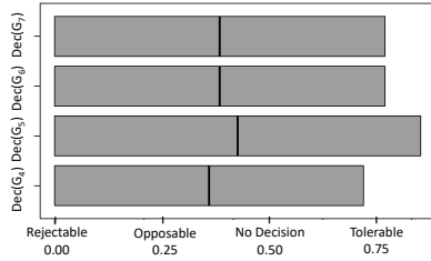
Fig. 8. Decision sensitivity on the top goal G_1
