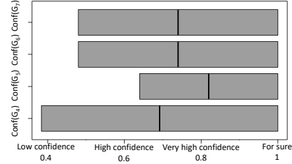
Fig. 9. Confidence sensitivity on the top goal G_1
