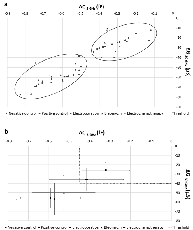
Fig. 8. Position of the different measurements of THP-1 cells undergoing different treatments, in the complex plane ( \Delta C_{5\text{GHz}} , \Delta G_{30\text{GHz}} ) (a) without and (b) with the standard deviations of measurement.
