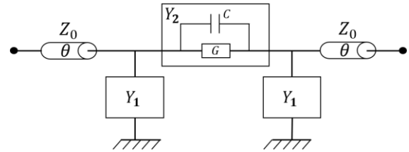
Figure 3: Electrical model of the device.
