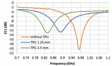
Fig. 4. Measurement of the return loss of UHF Antenna considering the effect of TPU layer.
