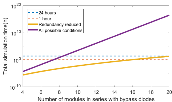
Figure 5 Time estimation to complete the sweep of 20 irradiation level per module for N modules in series
