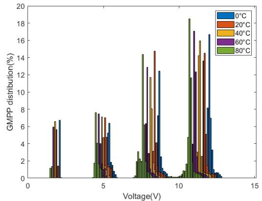
Figure 7 GMPP probability distribution of PV array consisting of 4 modules in series with 4 bypass diodes (real irradiation profile measurements)
