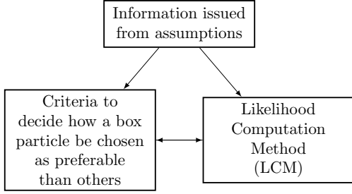
Fig. 1. Likelihood computation methodology diagram
