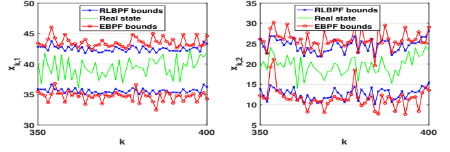
Fig. 2. RLBPF versus EBPF
