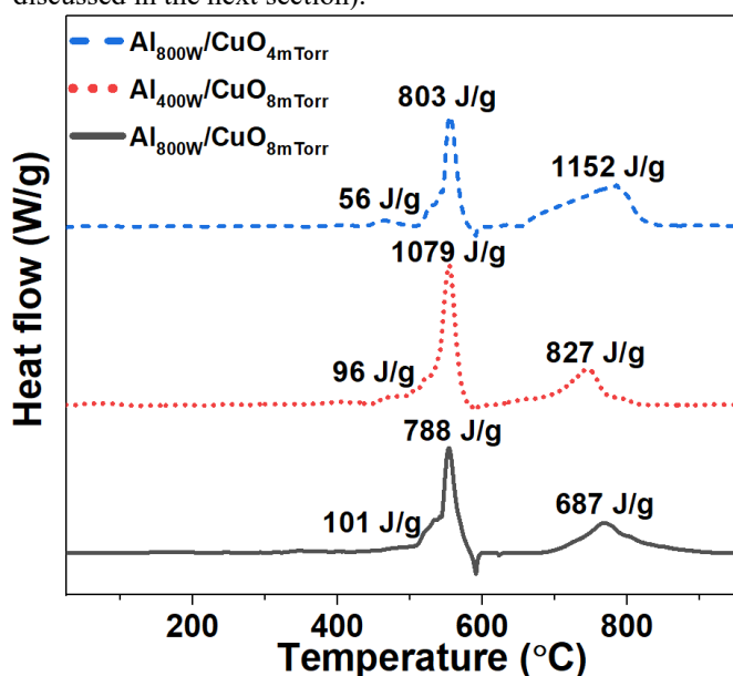
Figure 5: DSC traces from the as-deposited multilayers: \text{Al}_{800\text{W}}/\text{CuO}_{8\text{mTorr}} , \text{Al}_{400\text{W}}/\text{CuO}_{8\text{mTorr}} and \text{Al}_{800\text{W}}/\text{CuO}_{4\text{mTorr}}
