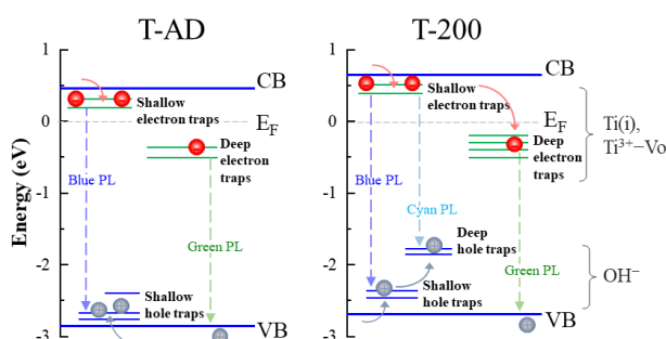
Fig. 8 Band gap scheme with localized intermediate traps of electron and holes in TiO 2 thin films T-AD and T-200. PL radiative recombination are represented by dashed lines. Electron traps are created by the presence of Ti 3+ species associated to Ti interstitials Ti(i) and oxygen vacancy Vo located on Ti 3+ sites, whereas hole traps are associated to OH - radicals adsorbed on the surface.
