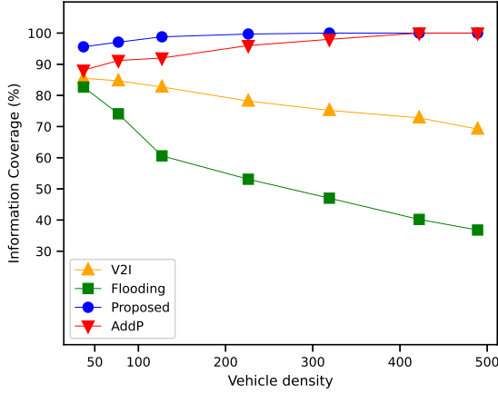
Figure 6: Information Coverage - Toulouse
