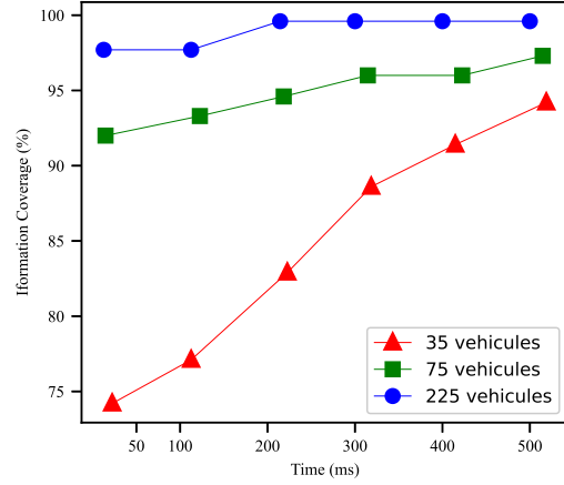
Figure 7: Information Coverage - Toulouse
