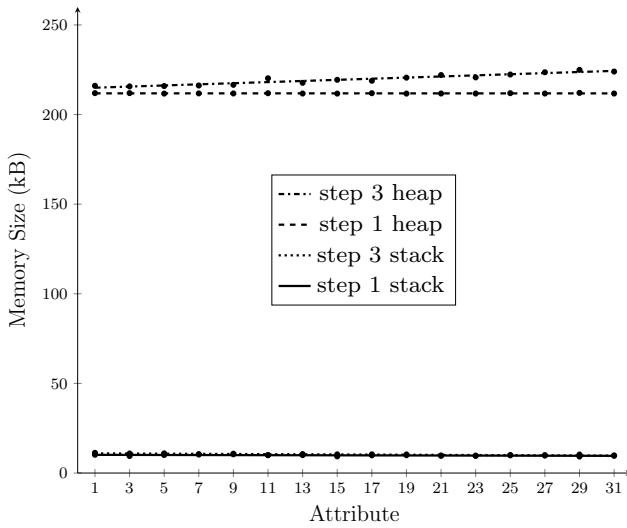
Fig. 12 Step 3 average maximum heap and stack size w.r.t the number of attribute for a 64 bytes data
