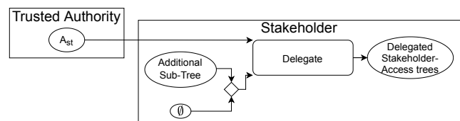
Fig. 7 Delegated access tree generation method
