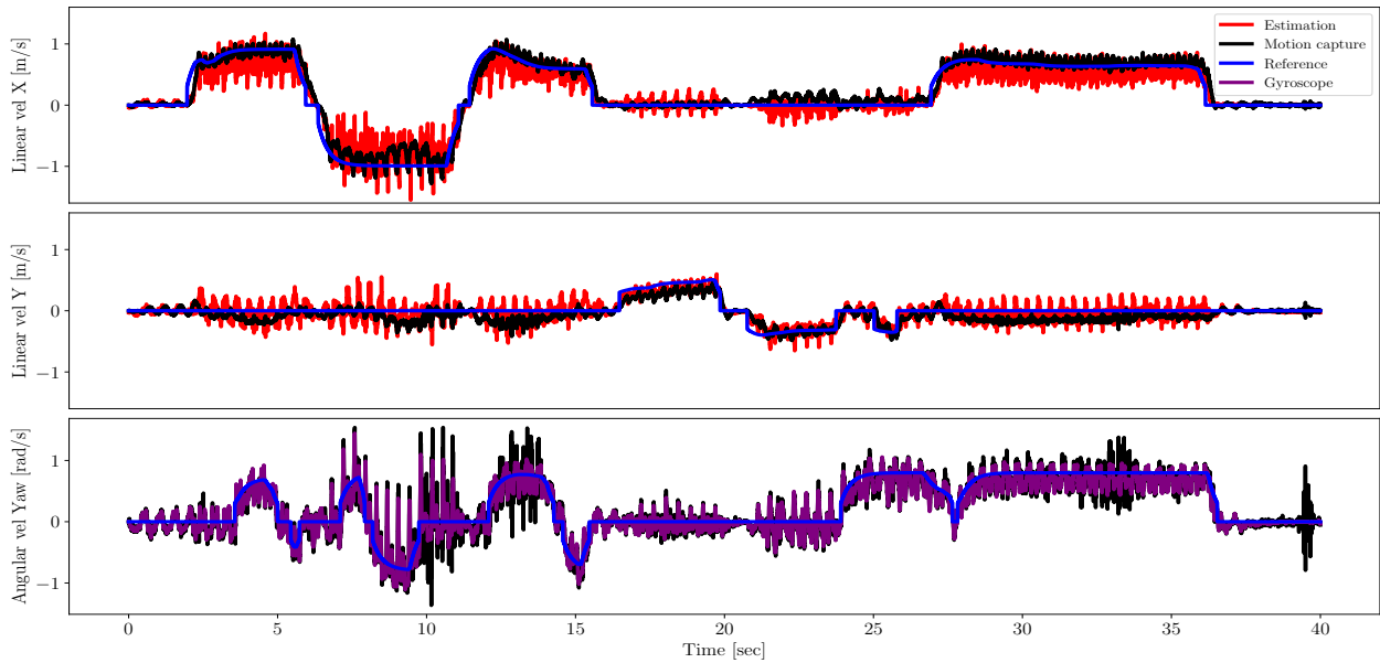
Figure 3. Plot of the 3D velocity command controlled by a gamepad to command the real robot in blue. The red curve plots the output of the state estimation. The black plot is the motion capture of the real solo12 to convey the ground-truth base velocity. The purple plot is the yaw velocity estimate from the gyroscope in the IMU. The x-axis shows time in seconds
