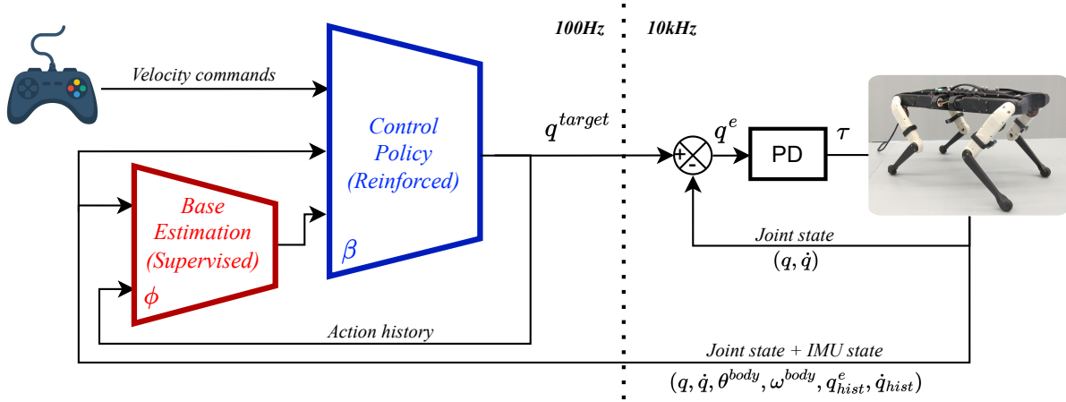
Figure 2. Summary of the control scheme shows the policy network, base estimation network and the low level control setup on the real robot
