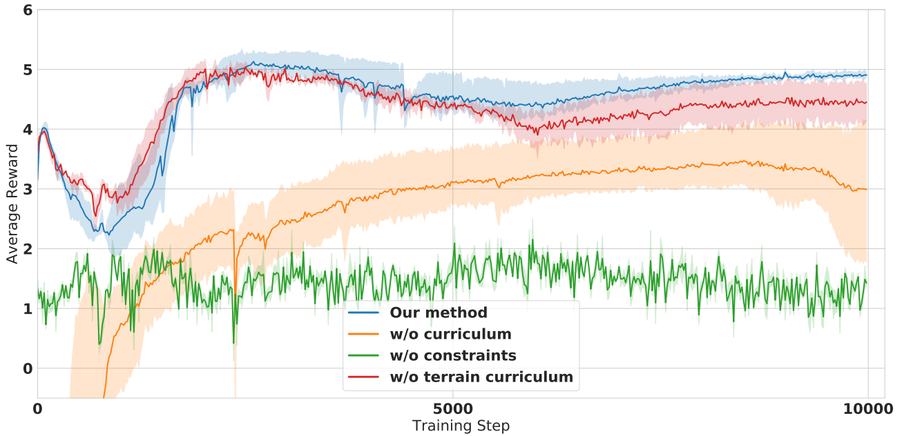
Figure 5. Plot of the average rewards over training steps for different setups. Each curve is averaged over three random seeds of the same experiment
