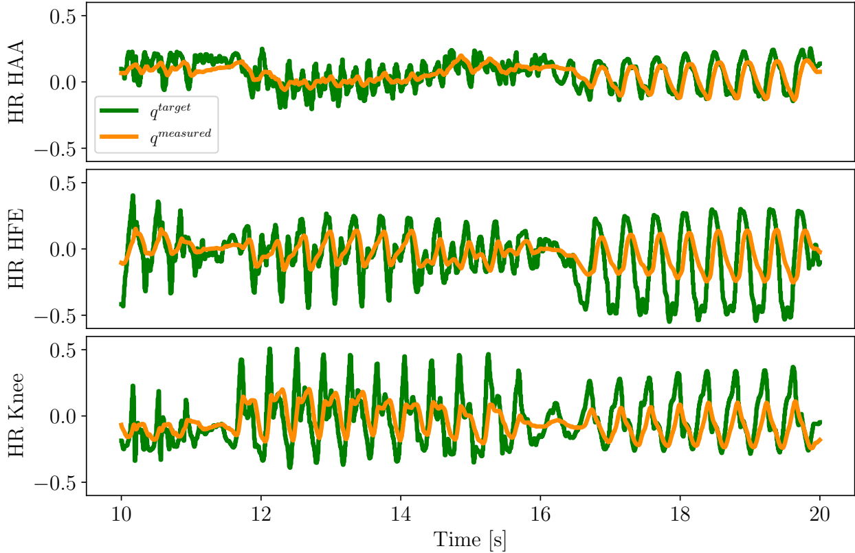
Figure 4. Plot of the desired joint angle command vs. the measured joint angles over a random run for the hind right leg. HFE stands for Hip-Flexion-Extension and HAA stands for Hip Aduction-Abduction
