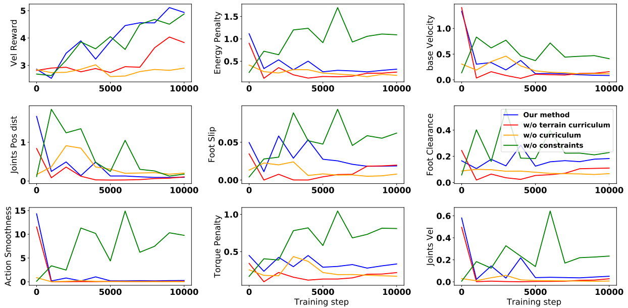
Figure 6. Plot of the separate reward penalties of the different curriculum settings over training steps
