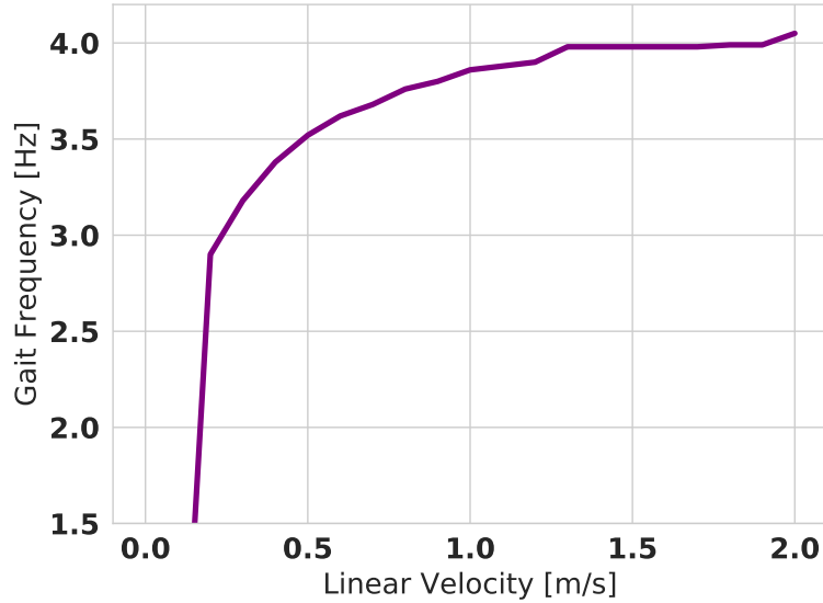
Figure 7. Plot of the gait frequency as a function of the linear velocity command
