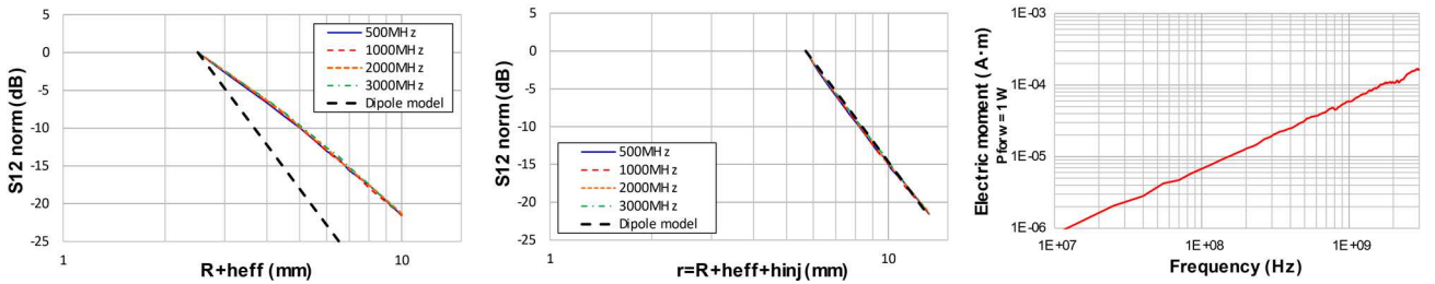
Fig. 3. Extraction of the E-field injection probe characteristics: normalized S_{12} vs. R+h_{eff} (left), adjustment of h_{inj} (center), electric moment (right)
