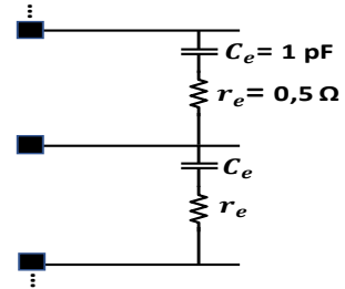
Fig. 7. High frequency model of the differential HP protection architecture
