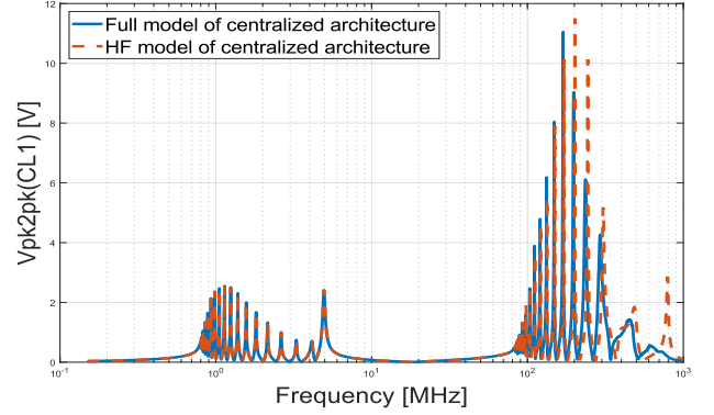
Fig. 6. Centralized architecture high frequency model validation.
