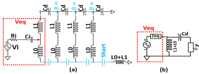
Fig. 4. Simplification of PCB model from Config B. (a) removal of C_L and R_b . (b) simplified model using Z_\beta
