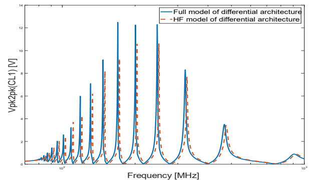
Fig. 8. Differential architecture high frequency model validation.
