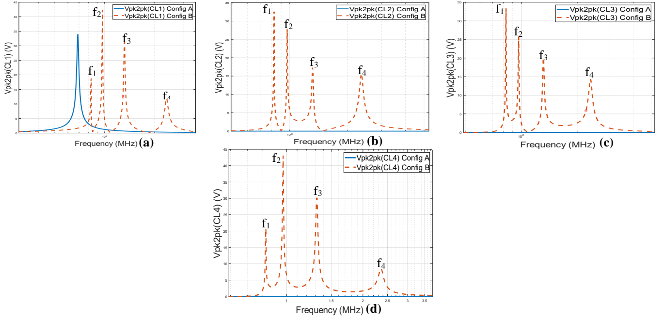
Fig. 3 V_{pk2pk}(C_{Li}) simulation results as a function of the injected frequency and comparing Config A with B. In the exception of the shown frequency range, the two curves of each graph fit together. (a) V_{pk2pk}(C_{L1}) in Config A and B. (b) V_{pk2pk}(C_{L2}) in Config A and B. (c) V_{pk2pk}(C_{L3}) in Config A and B. (d) V_{pk2pk}(C_{L4}) in Config A and B.
