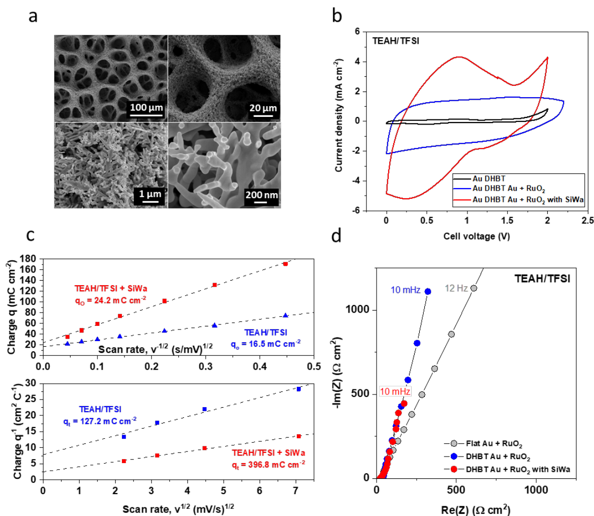
Fig. 3. Electrochemical performance \text{RuO}_2 MSC using interdigitated porous DHBT Au substrate characterised in neat TEAH/TFSI and SiWa doped TEAH/TFSI; a. Scanning electron microscopy (SEM) images at different magnification of DHBT Au substrate with \text{RuO}_2 deposition; b. Comparison of CVs with the bare DHBT Au and after \text{RuO}_2 deposition at a scan
