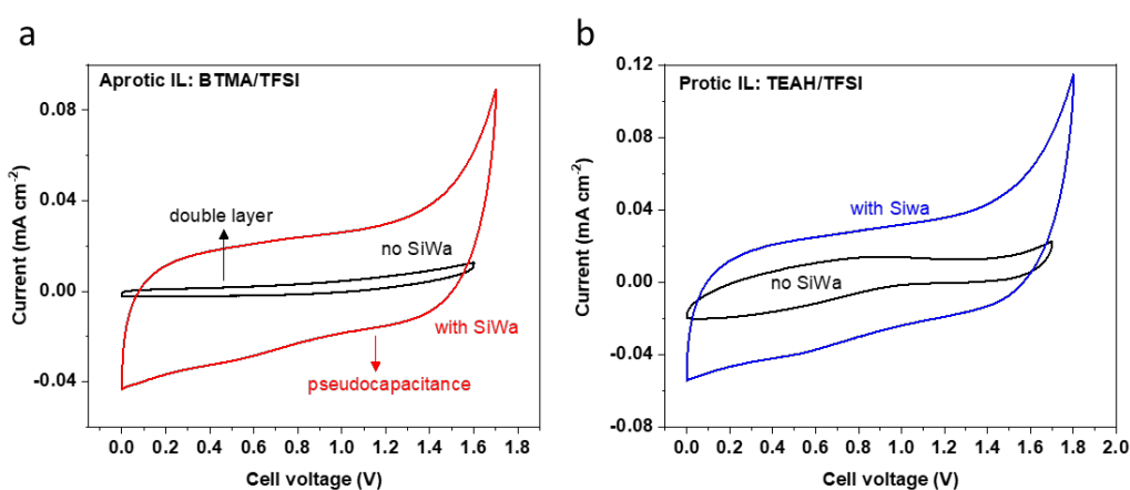
Fig. 2. Capacitive behaviour of protic and aprotic IL based on TFSI anion for RuO 2 MSCs using flat substrate in ILs with SiWa doping (10 wt%). a. CV curves (100 mV s -1 ) in an aprotic ionic-liquid, butyl-trimethyl ammonium trifluoromethane sulfonyl imide (BTMA/TFSI) before and after SiWa doping; b. CV curves using TEAH/TFSI before and after SiWa doping.
