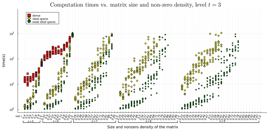
Fig. 2 This is a similar plot to Fig. 1 but now for level t=3 of each of the hierarchies. By omitting markers we indicate that the corresponding computations either exceeded memory constraints or took longer than 10^3 seconds
