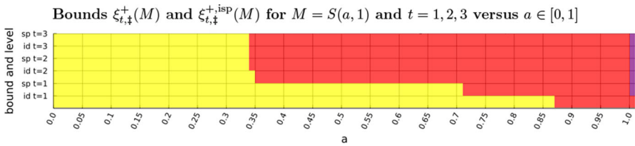
Fig. 3 This figure shows \xi_{t,\ddagger}^+(S(a, 1)) and \xi_{t,\ddagger}^{+,isp}(S(a, 1)) computed at levels t = 1, 2, 3 with a ranging from 0 to 1 in increments of 0.01. The colour indicates a lower bound on the obtained numerical value: yellow, red and purple show the bound is at least 2, 3, and 4, respectively. So a red square at a = 0.35 and “sp t=2” means \xi_{2,\ddagger}^{+,isp}(M) \geq 3
