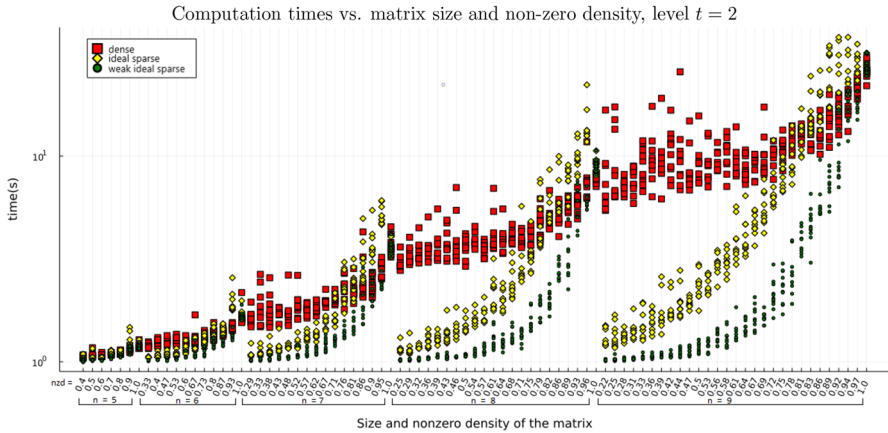
Fig. 1 Scatter plot of the computation times (in seconds) for the three hierarchies \xi_{2,\dagger}^{\text{cp}} (indicated by a red square), \xi_{2,\dagger}^{\text{cp,isp}} (indicated by a yellow losange), \xi_{2,\dagger}^{\text{cp,wisp}} (indicated by a green circle) against matrix size and non-zero density for 850 random matrices, generated using the above described procedure. The matrices are arranged in ascending size ( n = 5, 6, 7, 8, 9 ) and then ascending non-zero density, ranging from the minimal density needed to have a connected support graph up to a fully dense matrix ( \text{nzd} = 1 )
