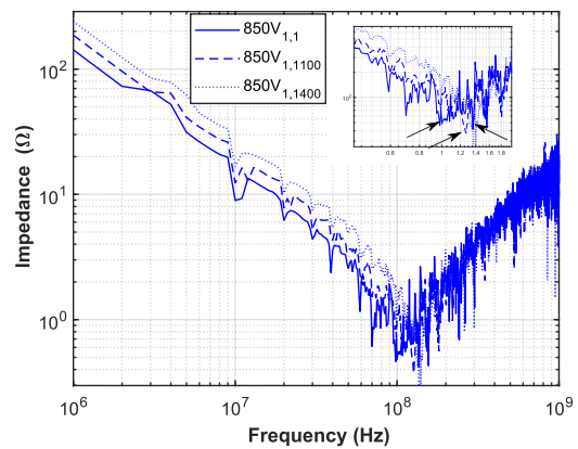
Fig. 8. Complex impedance of the X7R capacitor after
