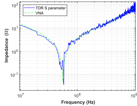
Fig. 2. Comparison between VNA and TLP-based TDR (100 V) measurements on the 1 nF C0G capacitor
