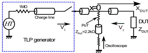
Fig. 1. Schema of TLP-based TDR measurement method
