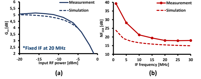
Fig. 7. Mixer with AND gates (a) Measured G_{cv} compression curve at a f_{RF} of 78 GHz (b) Measured NF_{SSB} at a f_{RF} of 78 GHz.
