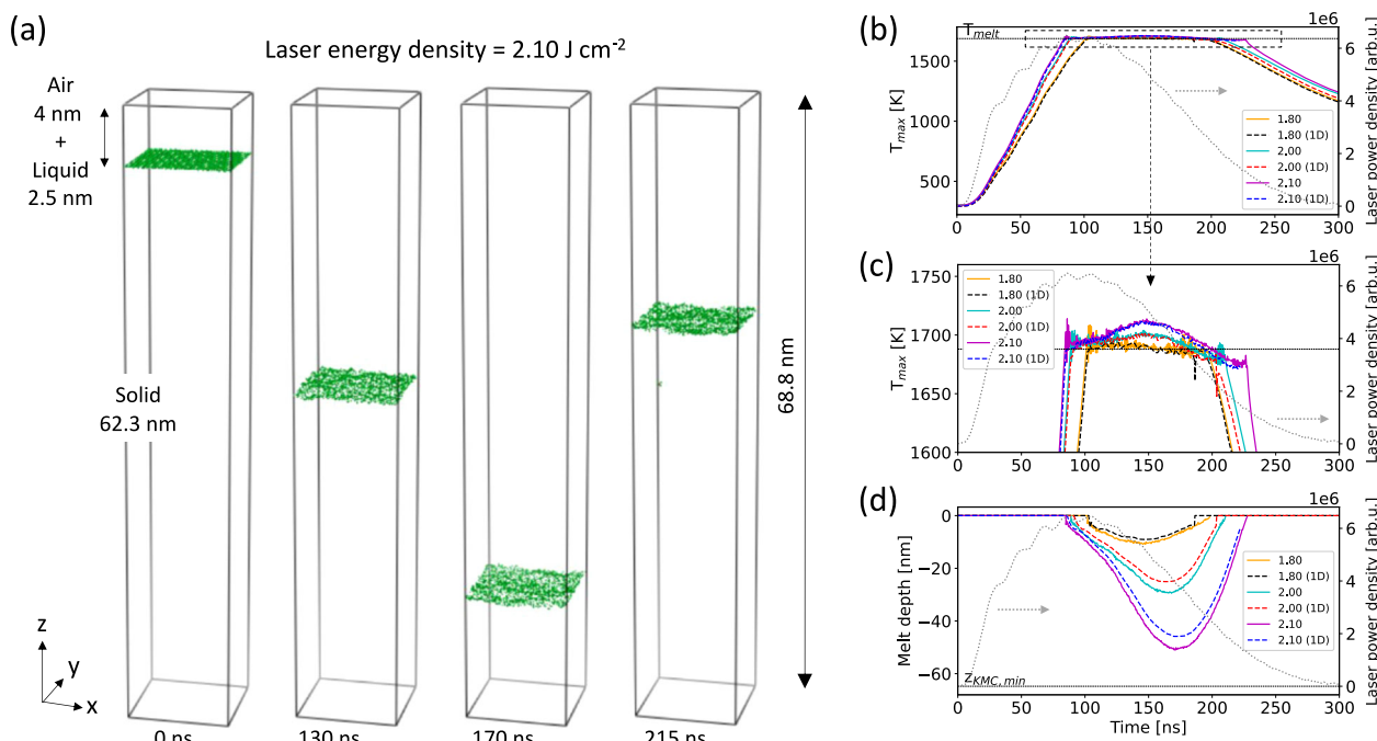
Fig. 4 FEM-KMC simulations of Si(100) laser annealing in the homogeneous nucleation case and comparison with 1D phase field. a KMC box containing all undercoordinated solid atoms (green), identifying the solid–liquid Si interface at t = 0, 130, 170, and 215 ns upon irradiation with a laser energy density of 2.1 \text{ J cm}^{-2} (see also Supplementary Movie 1). b Maximum T value in the FEM mesh as a function of time (solid lines), for laser energy densities of 1.8, 2.0, and 2.1 \text{ J cm}^{-2} , in comparison with the results of 1D phase-field model (dashed lines) using the same geometry and optical parameters. The power density of the laser pulse over time is also shown as black dotted line. c Zoom of the curves in (b) around T_M . d Variation of melt-depth over time for the same fluences (solid lines), in comparison with the results of the 1D phase-field model (dashed). The former are extracted as average z coordinate of solid Si atoms at the interface at the end of every KMC step. The maximum accessible depth for melting z_{KMC} in the KMC model is also indicated.
