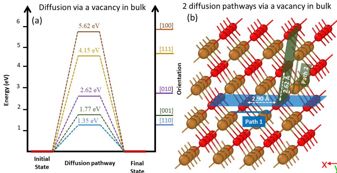
Figure 3. (a) Energetics (activation energies calculated using the CI-NEB method) and (b) bulk CuO atomistic view of oxygen migration path through oxygen vacancy sites. In (b), the two possible oxygen migration pathways are colored: in blue for the pathway following the [110] direction and, in green for the pathway following the [001] direction. The red and light brown balls represent oxygen and copper atoms, respectively.
