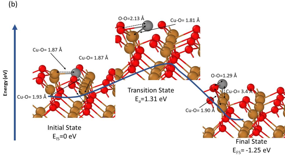
Figure 2. Creation of surface oxygen vacancy through oxygen migration towards nearest neighbors oxygen on (a) CuO(111) and (b) CuO(001) surfaces. Pathways as determined by CI-NEB. The red and light brown balls represent oxygen and copper atoms, respectively, while the gray ball represents the migrating oxygen atom.
