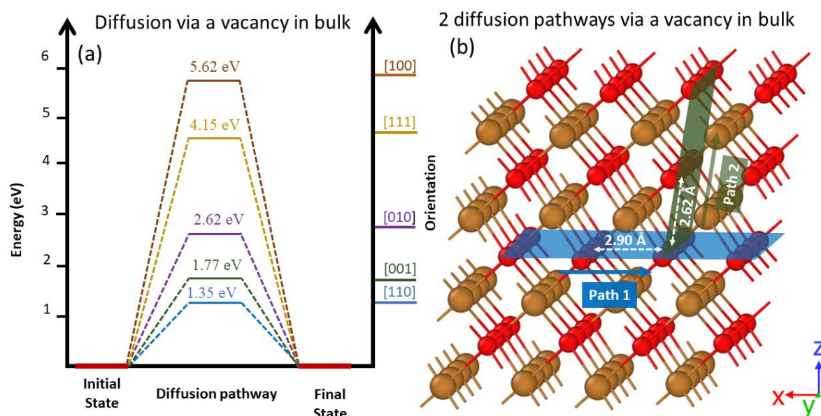
Figure 3. (a) Energetics (activation energies calculated using the CI-NEB method) and (b) bulk CuO atomistic view of oxygen migration path through oxygen vacancy sites. In (b), the two possible oxygen migration pathways are colored: in blue for the pathway following the [110] direction and, in green for the pathway following the [001] direction. The red and light brown balls represent oxygen and copper atoms, respectively.
