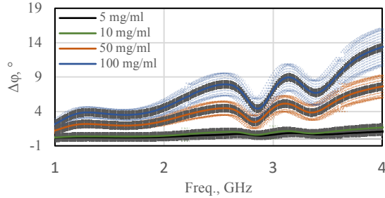
Fig. 4. The average values of differences of phase contrasts of measured S_{21} for the BSA solutions for different concentrations, with marked standard deviations
