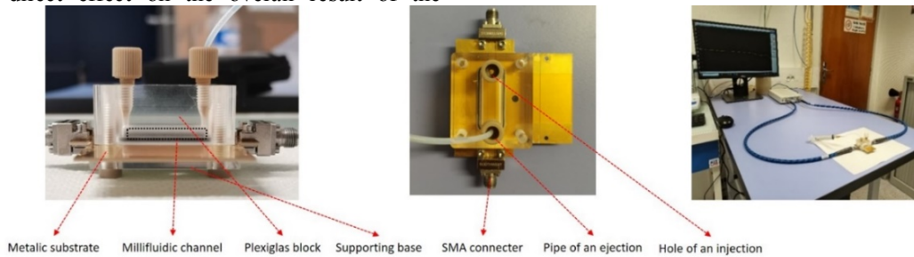
Fig. 2. Photographies of the millifluidic and microwave device, seen from the side (in the left) and from above (in the right), with the coplanar waveguide, the millifluidic channel, SMA connectors, Plexiglas block and the inlet and the outlet hole and pipe and an experimental test setup with the microwave millifluidic sensor
