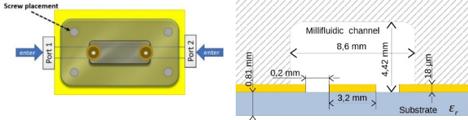
Fig. 1. Schematic of the simplified millifluidic and microwave sensor with two ports with dimensions. The coplanar waveguide is represented in yellow, whereas a plexiglas fluidic channel is placed on top.
