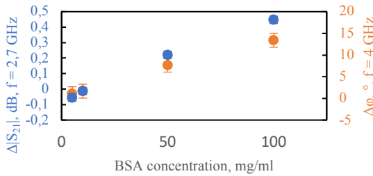
Fig. 5. Measured standard deviation and average modulus contrasts of S_{21} for each BSA solution versus concentration, at 2,7 GHz (in blue) and measured standard deviation and average phase of S_{21} for each BSA solution versus concentration, at 4 GHz (in orange)
