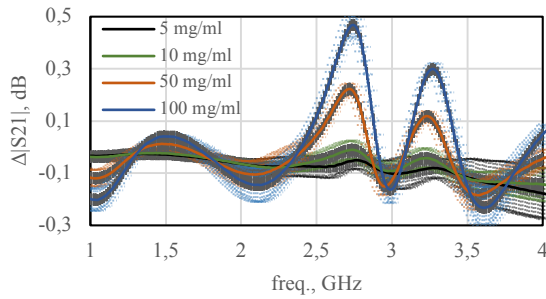
Fig. 3. The average values of differences of modulus contrasts of measured S_{21} for the BSA solutions for different concentrations, with marked standard deviations
