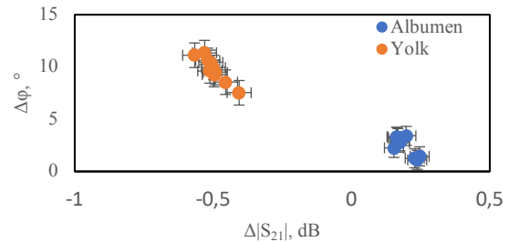
Fig. 6. Complex graph of S_{21} modulus on phase contrasts of 10 measurements for the yolk and the albumen of hen eggs with marked standard deviations at 3 GHz
