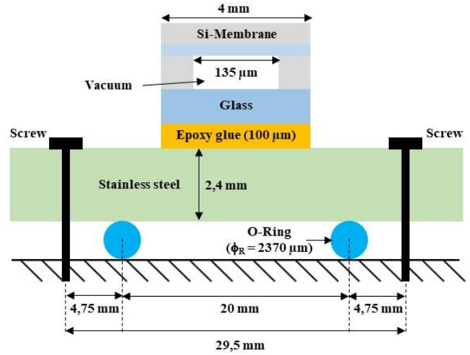
Figure 9. Cross section view of the device used for the simulation model.
