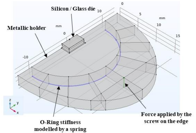
Figure 10. COMSOL 3D view of the half-simulated device. The membrane length is along x axis.
