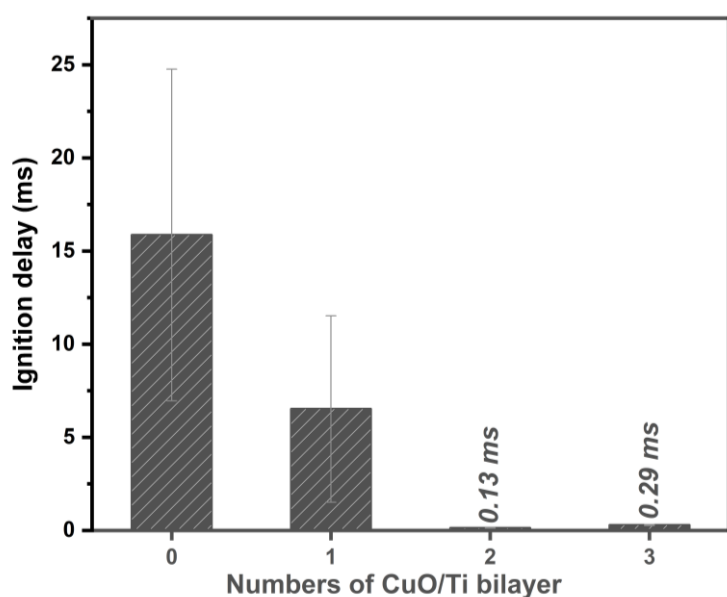
Figure 9. Ignition delay of (\text{CuO}/\text{Ti})_{x\text{BL}}/(\text{CuO}/\text{Al})_{(15-x)\text{BL}} nanolaminates ( x=0, 1, 2 , or 3 ).
