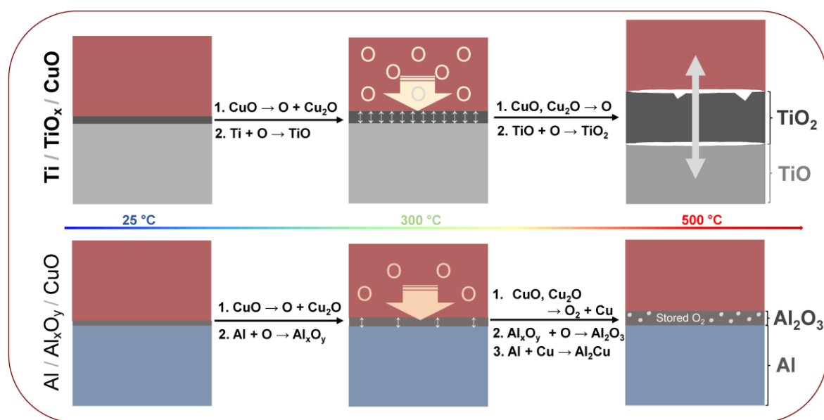
Figure 8. Schematic of the reaction mechanism of CuO/Ti compared with CuO/Al.
