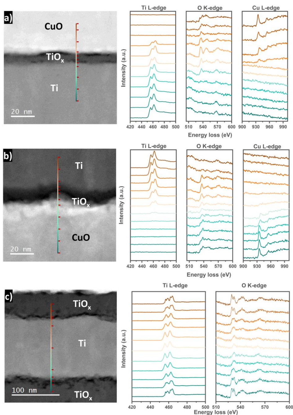
Figure 7. STEM-HAADF-EELS results of Ti-CuO (a) and CuO-Ti (b) annealed at 300 °C, and \text{TiO}_x -Ti- \text{TiO}_x annealed at 500 °C (c), showing Ti L_{2,3} , Cu L_{2,3} , and O k -edge.
