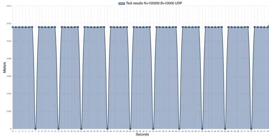
Fig. 8. Throughput on the n41 band with N = 0.1Mbits and B = 10kHz
