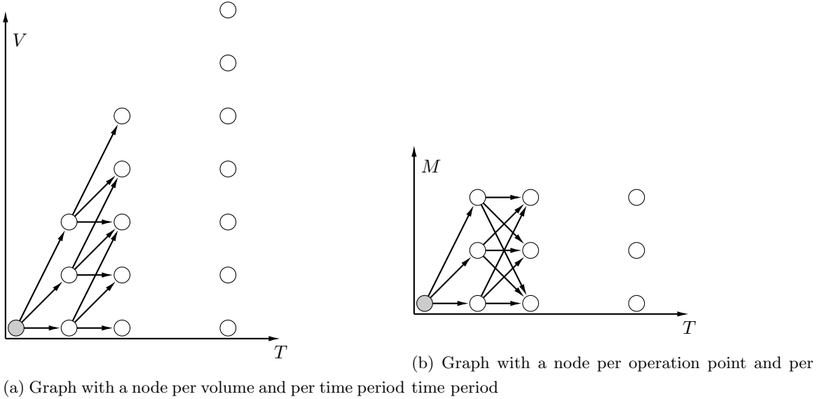
Figure 1: Graphical representations of the 1-HUC
