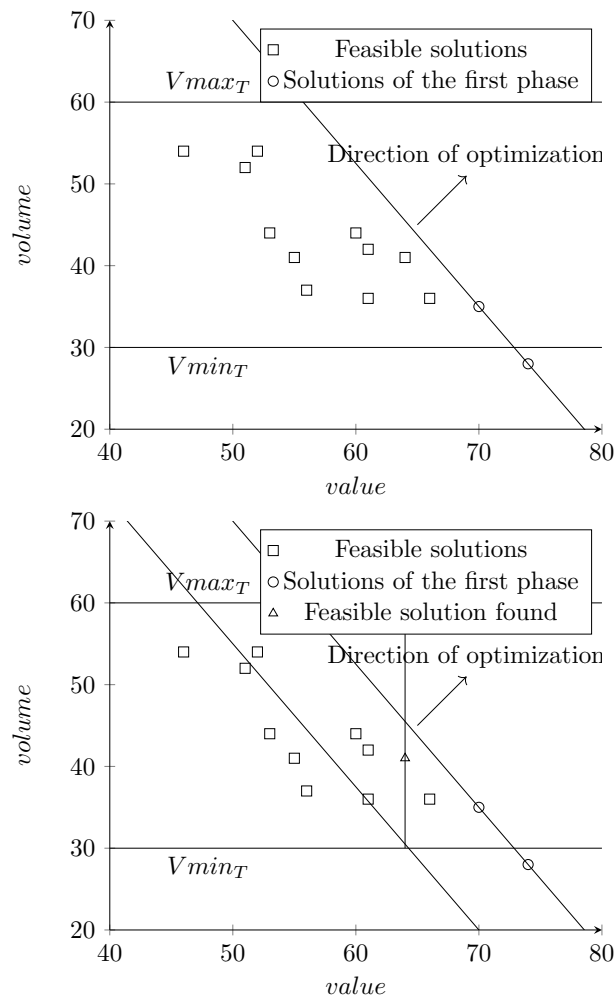
Figure 3: Representation of the solution search space during the algorithm
