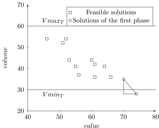
Figure 2: Pathological case to use a triangle
