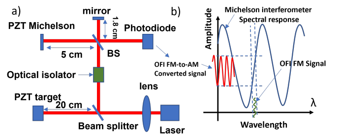
Fig. 1. Schematic diagram of: (a) the OFI system with OFI FM-to-AM conversion using a Michelson interferometer with a piezo-electric transducer (PZT) as target, and (b) OFI FM-to-AM conversion via the steep edge of the Michelson interferometer response used as a filter.
