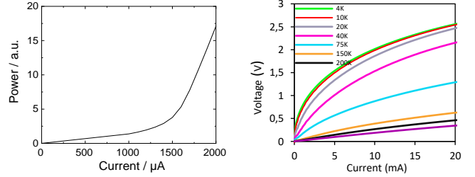
Left: Current-Output power curve around 4.2 K. Right: p-DBR mirror I-V curve as a function of temperature.
