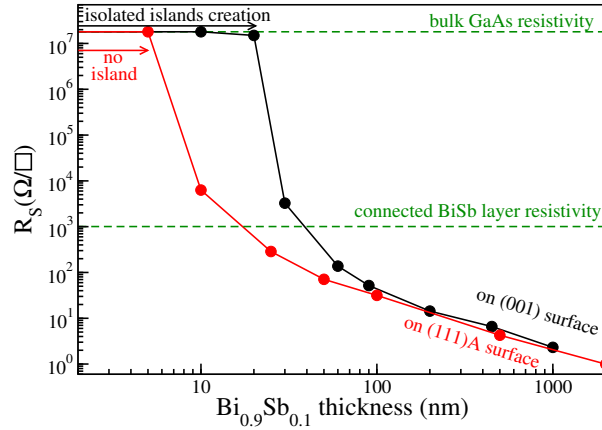
Figure 3: Variation of the sample resistivity for different Bi 0.9 Sb 0.1 thicknesses on the GaAs (001) (black) and GaAs (111)A (red) surfaces.
