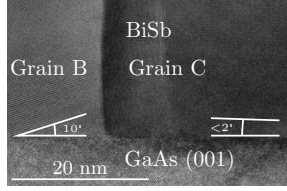
(a) Bi 0.9 Sb 0.1 deposited on GaAs (001) surface
