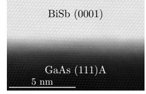
(b) Bi 0.9 Sb 0.1 deposited on GaAs (111)A surface
