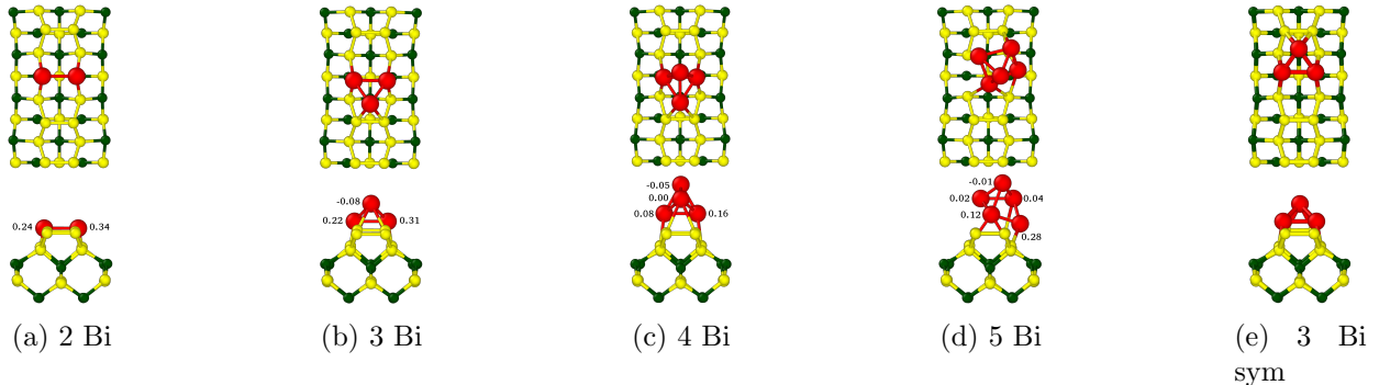
Figure 6: Most stable atomic configurations of the agglomeration of two to five Bi atoms on the GaAs (001). Structures 3 and 5 can exist symmetrically, and an example is given for structure 3 panel 6e. Variation of Bader charge is given on each adsorbed Bi atom in reference to the value of Bi in its pseudopotential.
