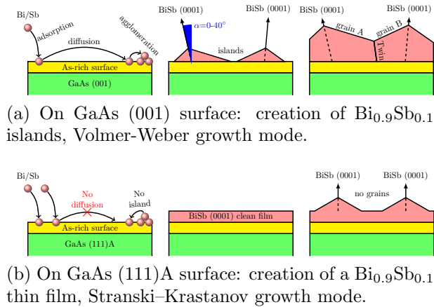
Figure 7: Schema of the two different growth modes.
