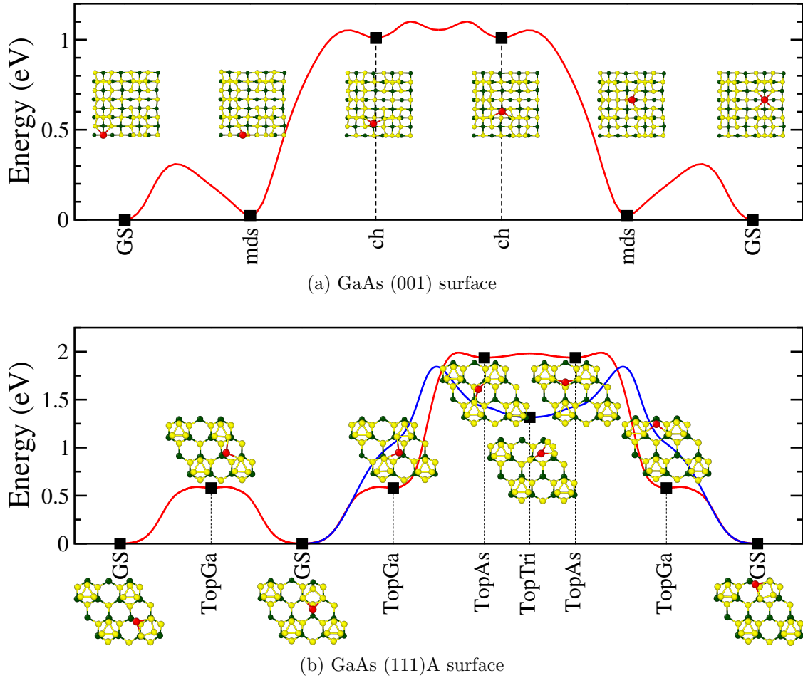
Figure 4: Minimum energy pathways of the Bi atom between the ground state positions above the (a) GaAs (001) and (b) GaAs (111)A surfaces. Red ball represent the adsorbed Bi atom.
