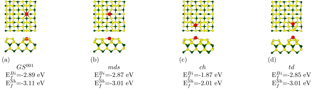
Figure 9: Stable adsorption sites on the GaAs (001) surface. Yellow, green and red spheres represent As, Ga and Bi/Sb atoms, respectively.
