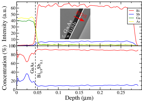
Figure 8: Variation of the energy dispersion spectroscopy (EDS) intensities for each atom type (top panel) while crossing the BiSb grain. The beam path is represented by the red arrow on the insert transmission electron microscopy (TEM) panel. The calculated Bi and Sb concentrations (bottom panel) are calculated from there respective intensities.
