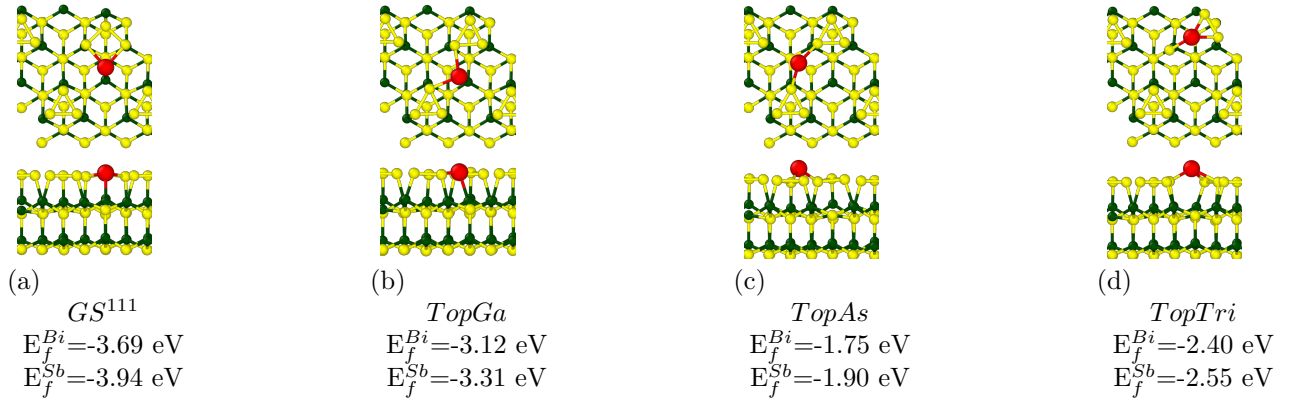
Figure 10: Stable adsorption sites on the GaAs (111)A surface. Yellow, green and red spheres represent As, Ga and Bi/Sb atoms, respectively.
