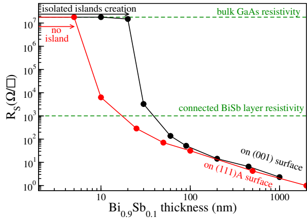
Figure 3: Variation of the sample resistivity for different \text{Bi}_{0.9}\text{Sb}_{0.1} thicknesses on the GaAs (001) (black) and GaAs (111)A (red) surfaces.
