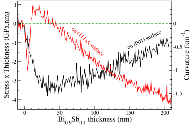
Figure 11: Stress \times thickness product (left axis), or wafer curvature (right axis), as a function of the deposited \text{Bi}_{0.9}\text{Sb}_{0.1} thickness on GaAs (001) (black line) or on GaAs (111)A (red line), at 215^\circ\text{C} (Bi flux of 4\times 10^{-7} Torr and Sb flux of 5\times 10^{-8} Torr for both growths).
