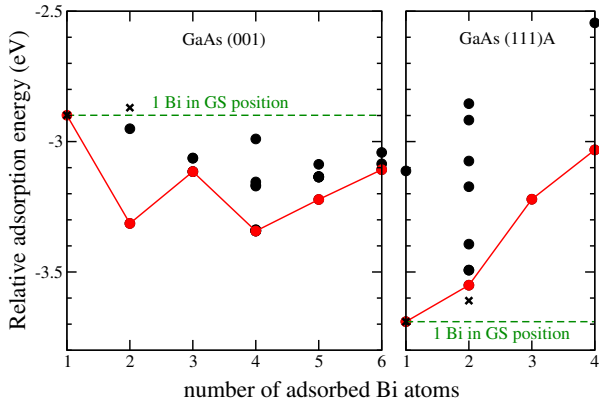
Figure 5: Relative adsorption energies ( E_{ad,rel}^n ) of the n Bi atoms on (left) the GaAs (001) and (right) the GaAs (111)A surfaces. Each dot corresponds to a structure where the atoms are agglomerated into islands, each cross to a structure where the atoms do not form islands, and the green line is the energy of the isolated ground state structure. The red dots correspond to the most stable agglomerated structures at a given Bi coverage that serve as energy reference for the next added atom.
