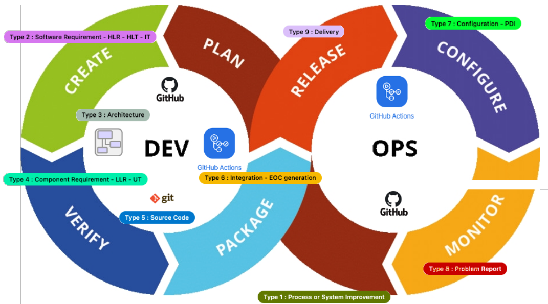
Figure 7 – Proposal of tool association to the different phases
