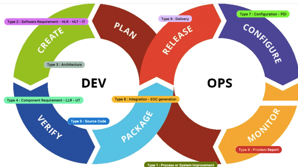
Figure 6 – Ticket implementation and continuous development
