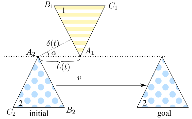
Fig. 5: Example of a single collision. Each body is a triangle A_iB_iC_i . Along the path, the triangle 1 (yellow stripes) is static. The triangle 2 (blue dots) moves from its initial position to its goal position with a constant velocity \mathbf{v} . Along the path, the lines (B_1C_1) , (B_2C_2) and (A_1A_2) are parallel. There is a single collision during the motion, which the algorithm generally fails to find.
