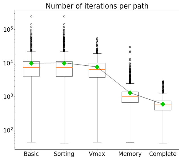
(a) Random Test Case: Box plot (log scale) of the number of iterations per path
