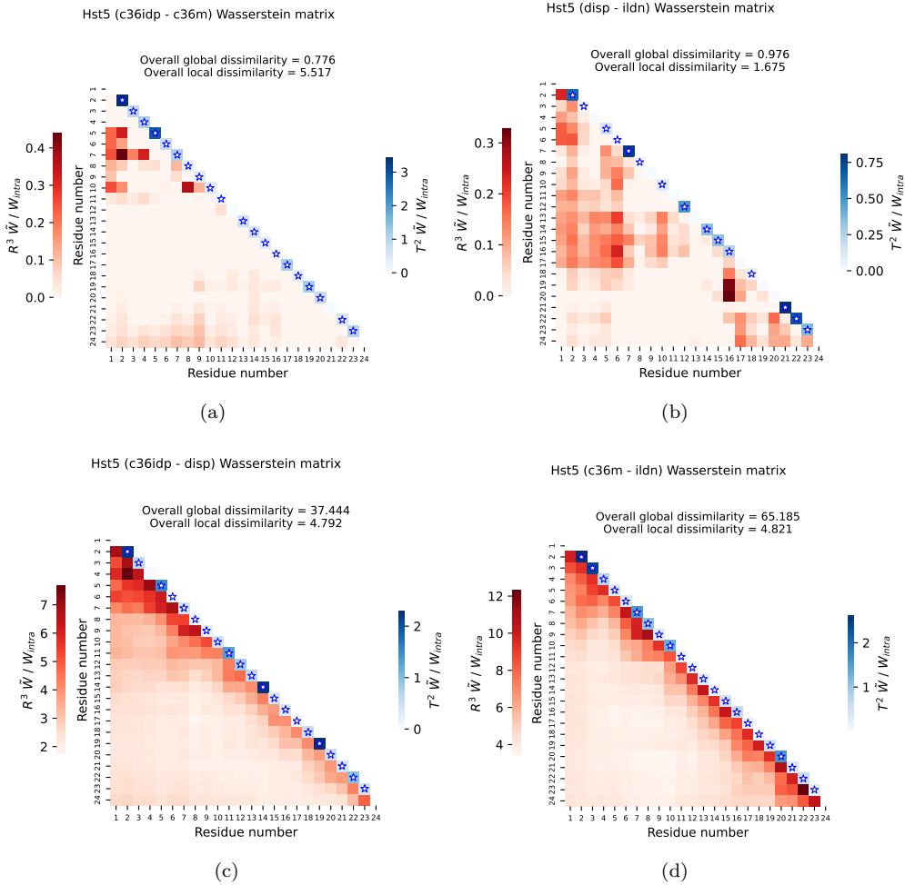
Figure 2: Comparison of Molecular Dynamics simulations of Hst5 ensemble using different force-fields. The color scale \bar{W}/W_{\text{intra}} corresponds to the score (10), representing the relative difference between the inter-ensemble distances and the uncertainty.
